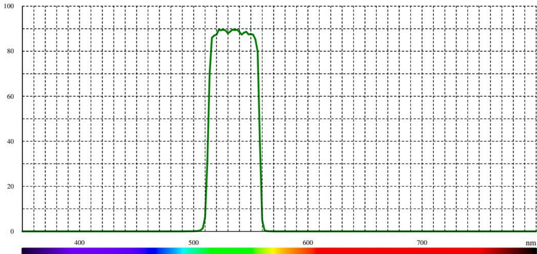
Typical transmission for BP 535/45 (LF101969)
