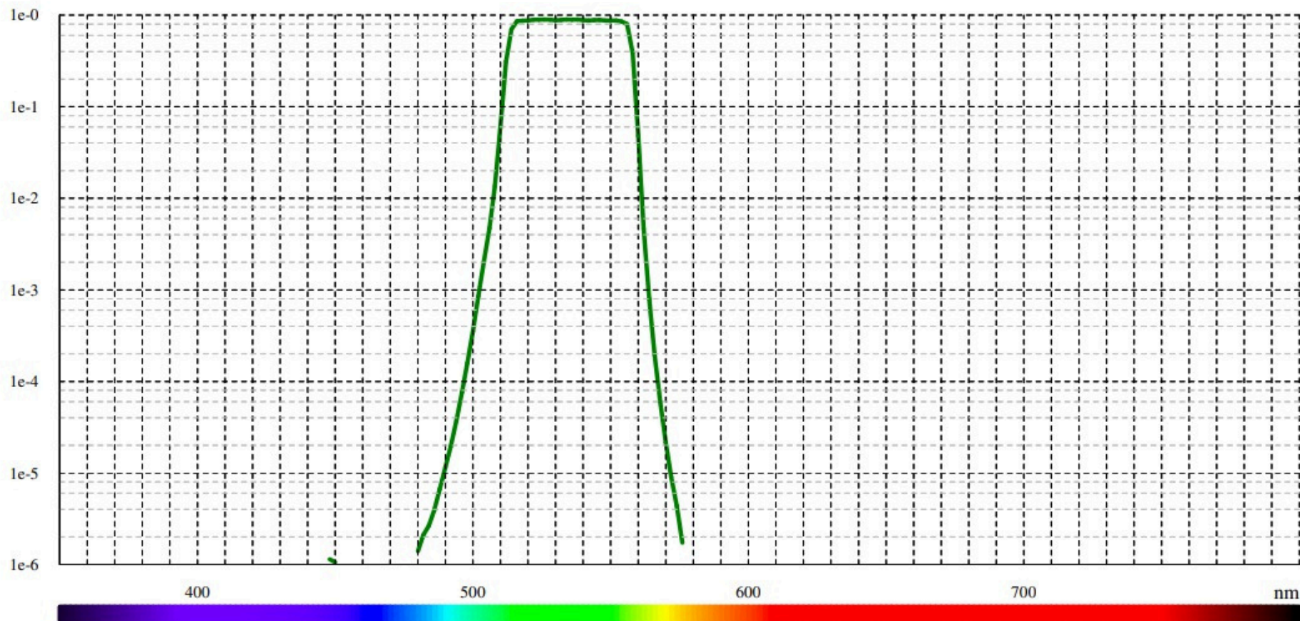
Typical transmission for BP 535/45 (LF101969)
