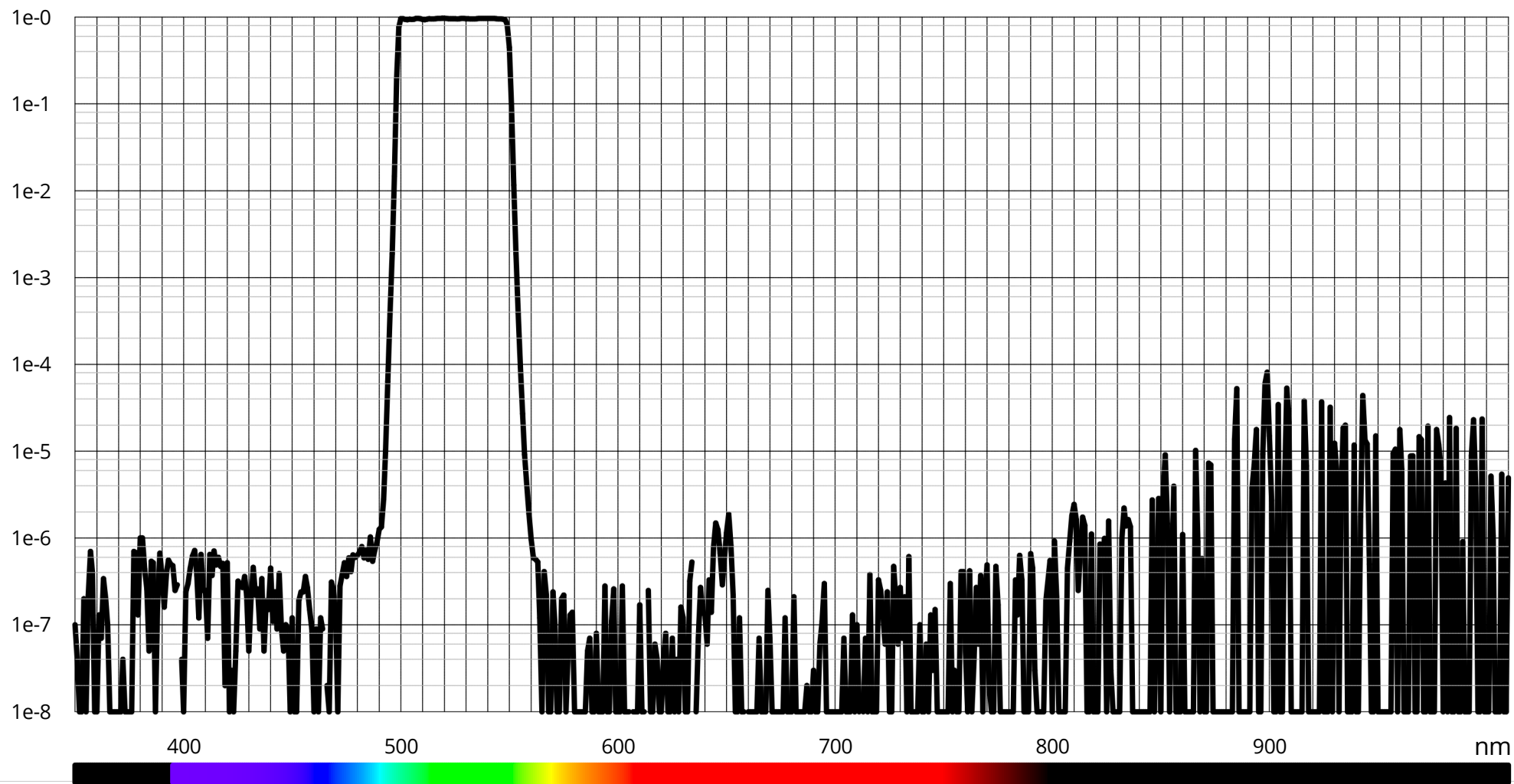
Typical transmission BP525-50 (LF101780)
