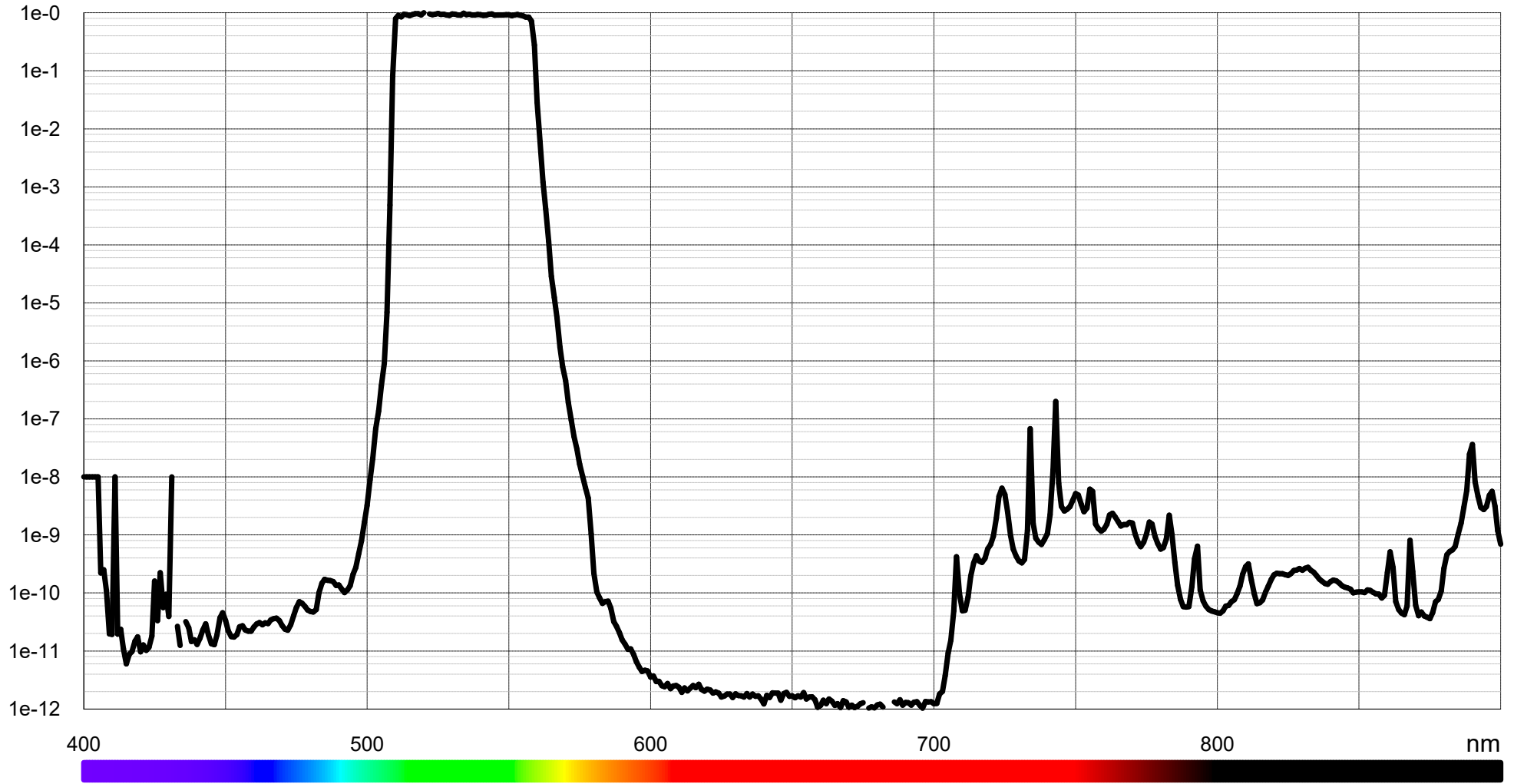
Typical transmission BP534-51 (LF104931)
