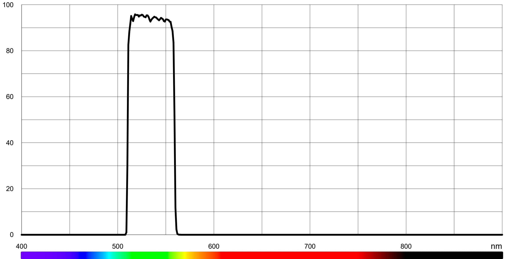
Typical transmission BP534-51 (LF104931)
