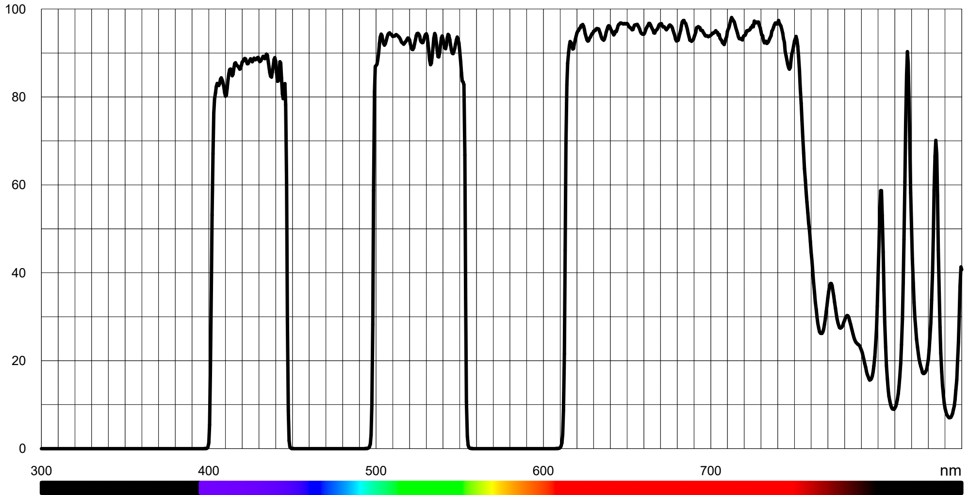
Typical transmission TBF 425 527 LP615 (LF104707)
