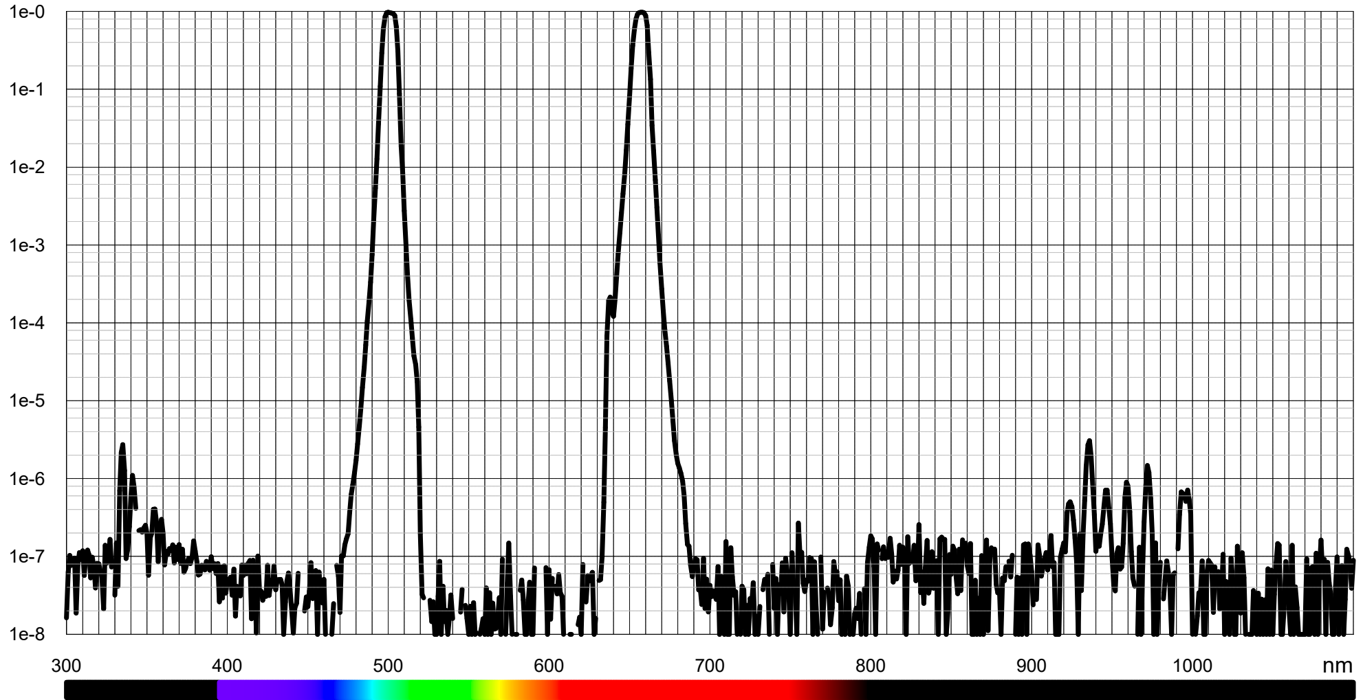
Typical transmission DBP O-III H-alfa (LF104691)
