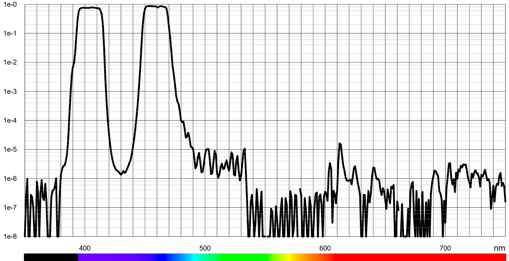
Typical transmission DBP 405 460 (LF104706)
