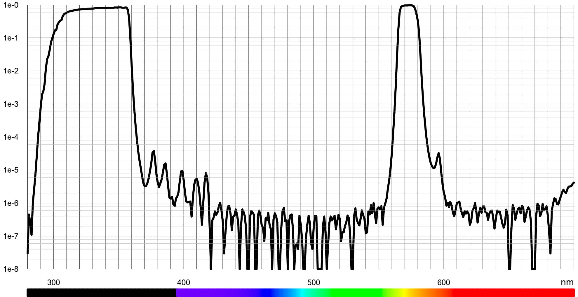
Typical transmission DBP 338 570 (LF104692)
