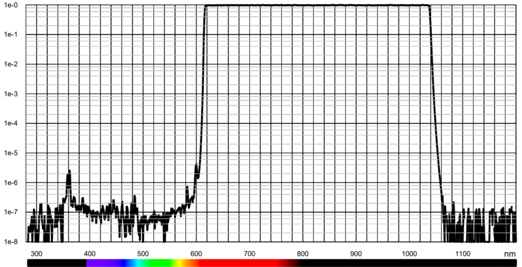
Typical transmission 615 nm - 1040 nm (LF104554)
