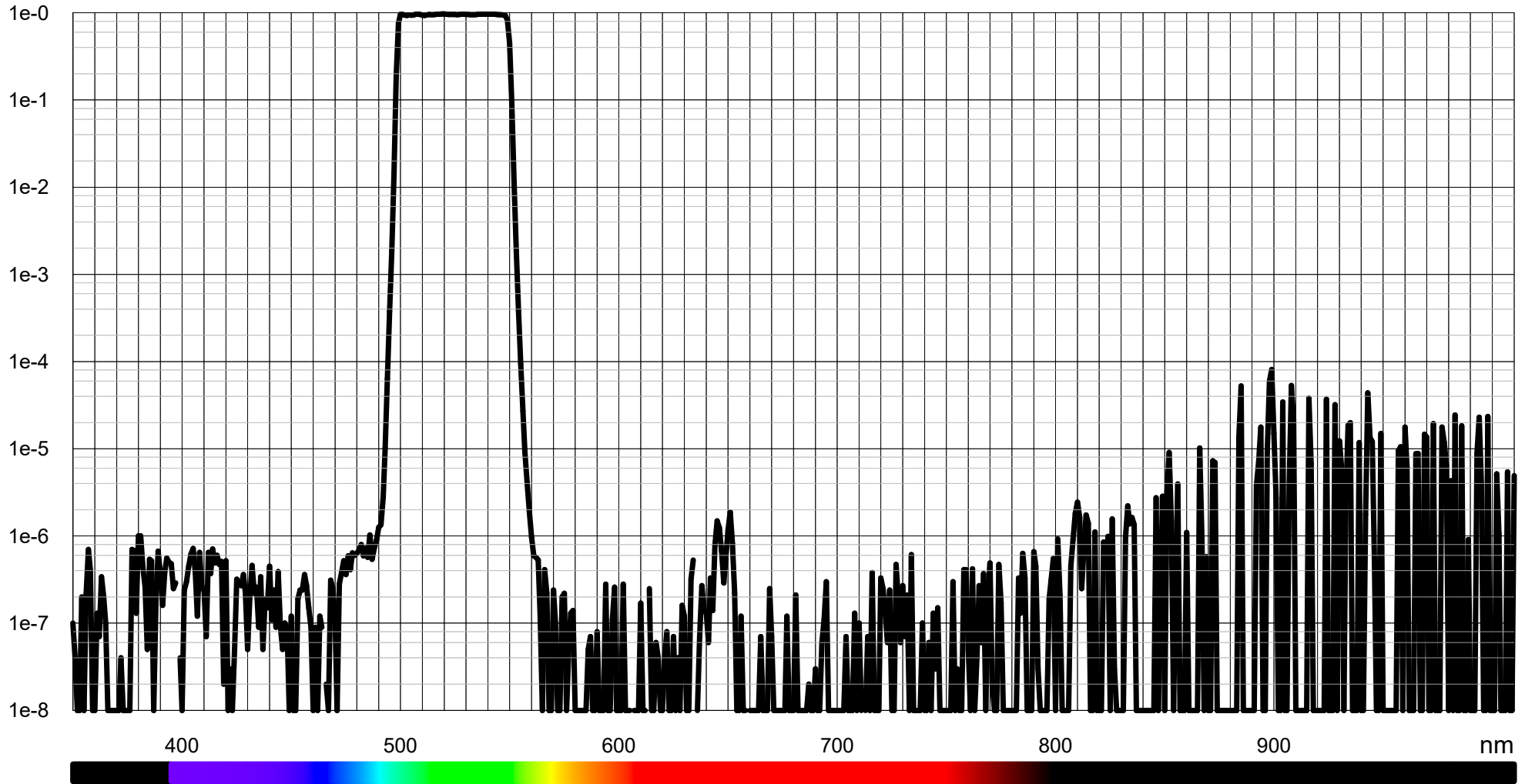
Typical transmission BP525-50 (LF121787)
