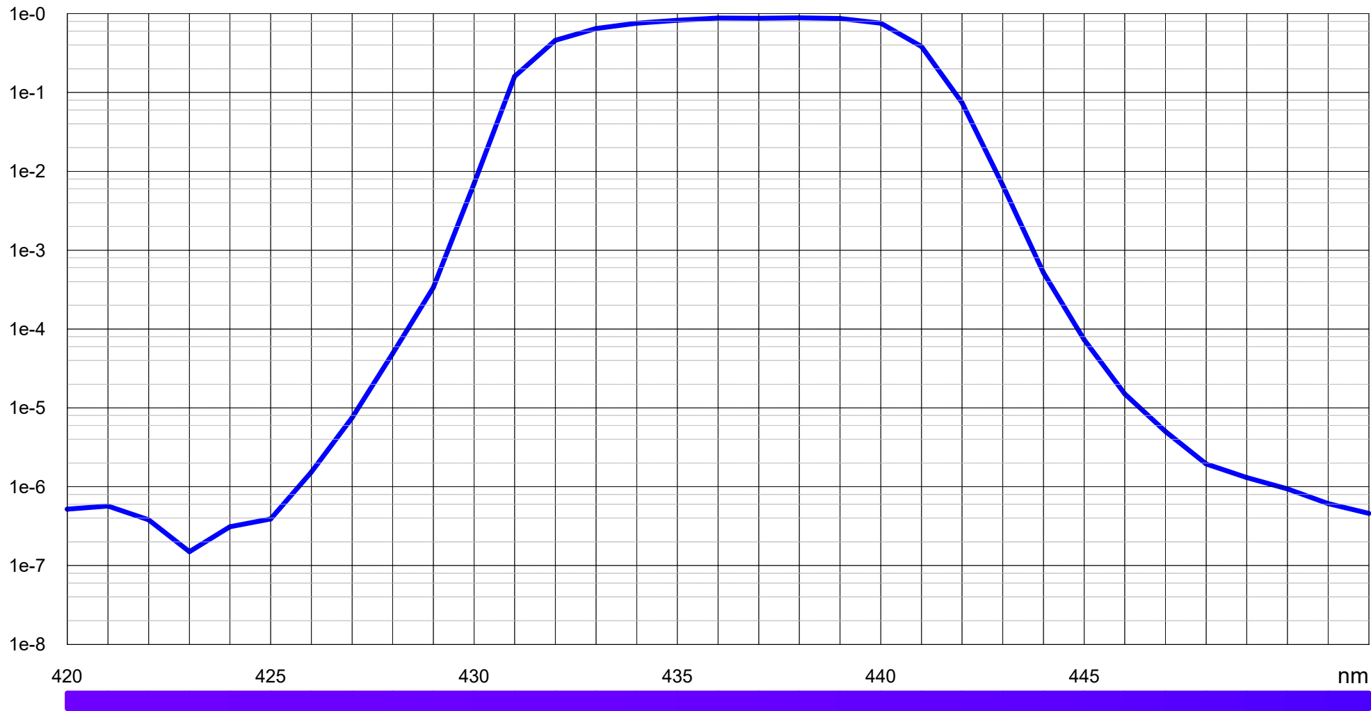
Typical transmission BP436/10 (LF101532)
