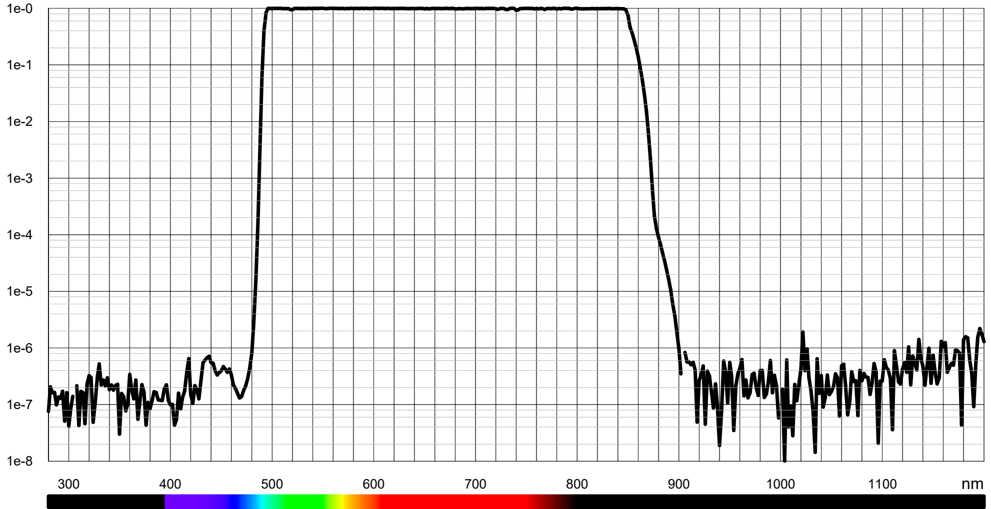
Typical transmission 490 nm - 850 nm (LF104553)
