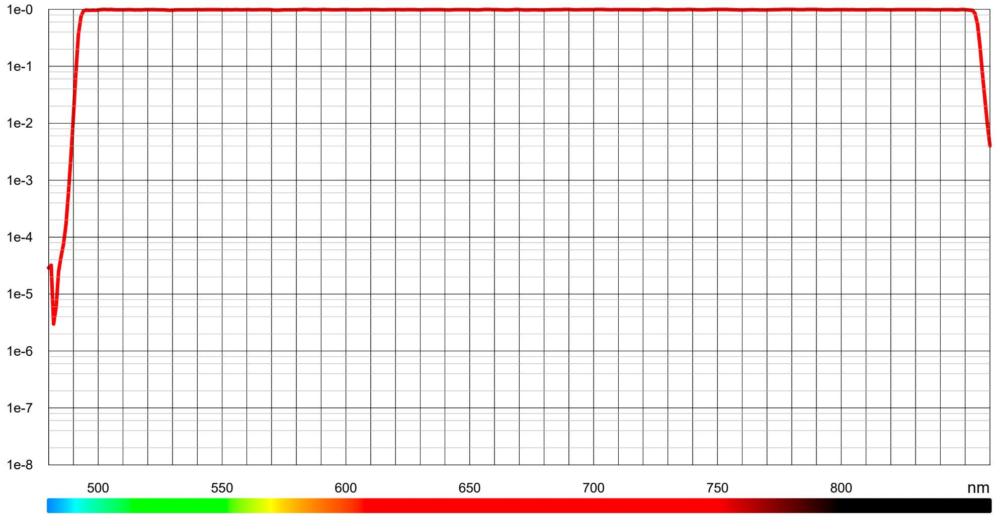
Typical transmission 490 nm - 850 nm (LF104553)
