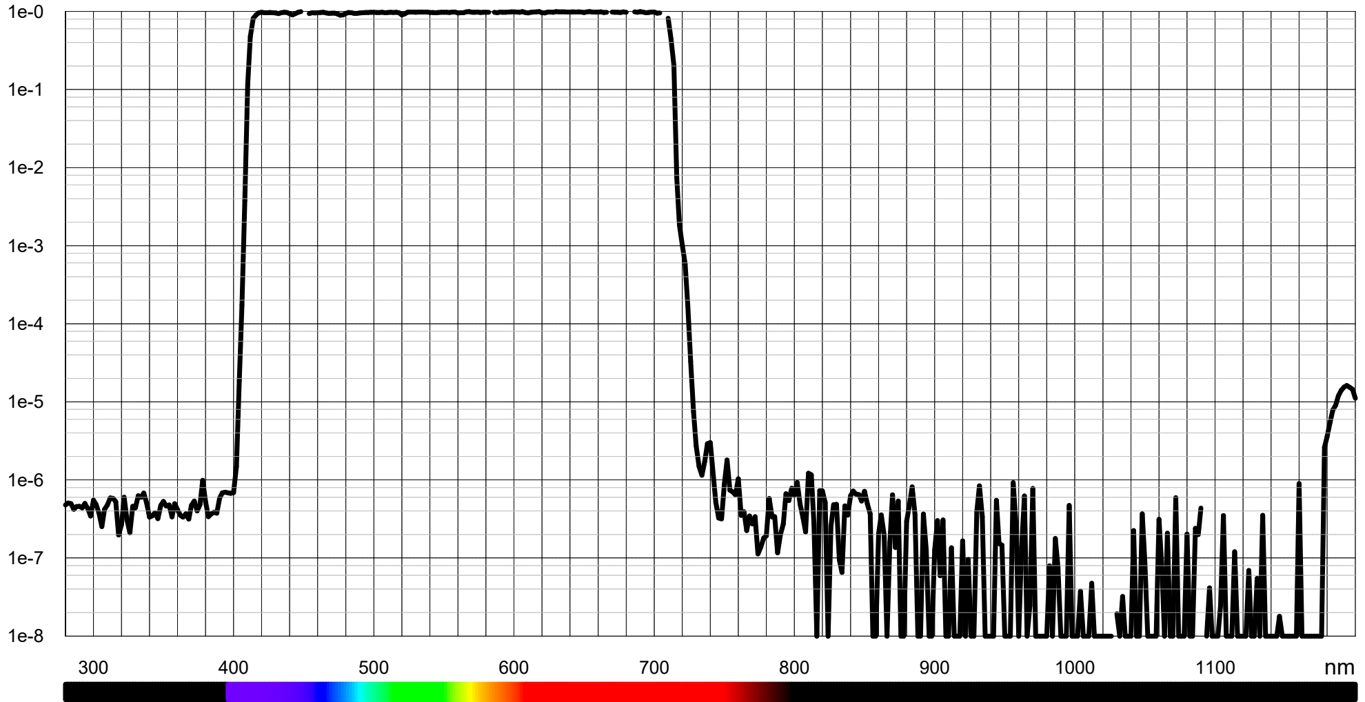
Typical transmission 410 nm - 710 nm (LF104552)
