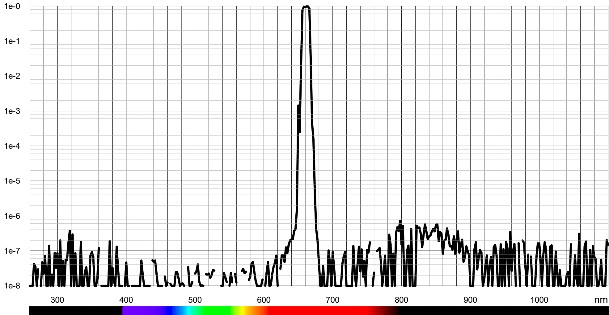
Typical transmission BP 661/12 (LF104544)
