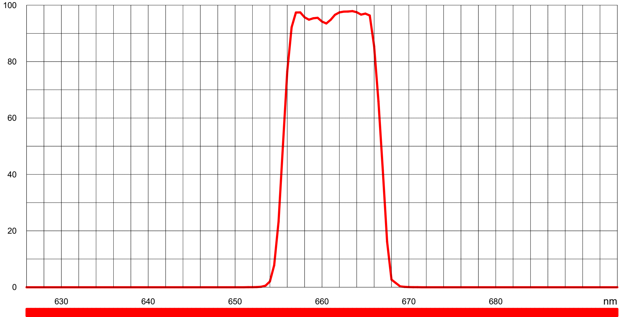
Typical transmission BP 661/12 (LF104544)
