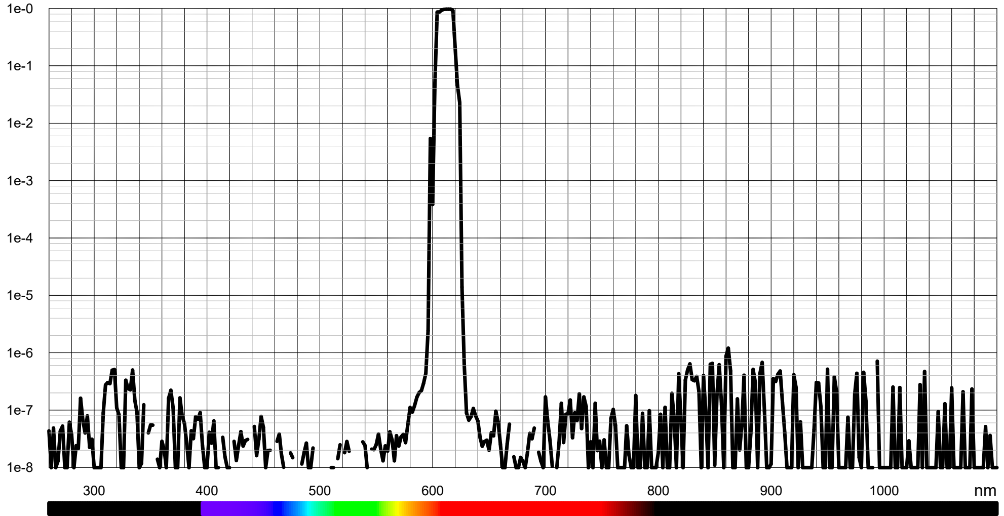
Typical transmission BP612/12 (LF104545)
