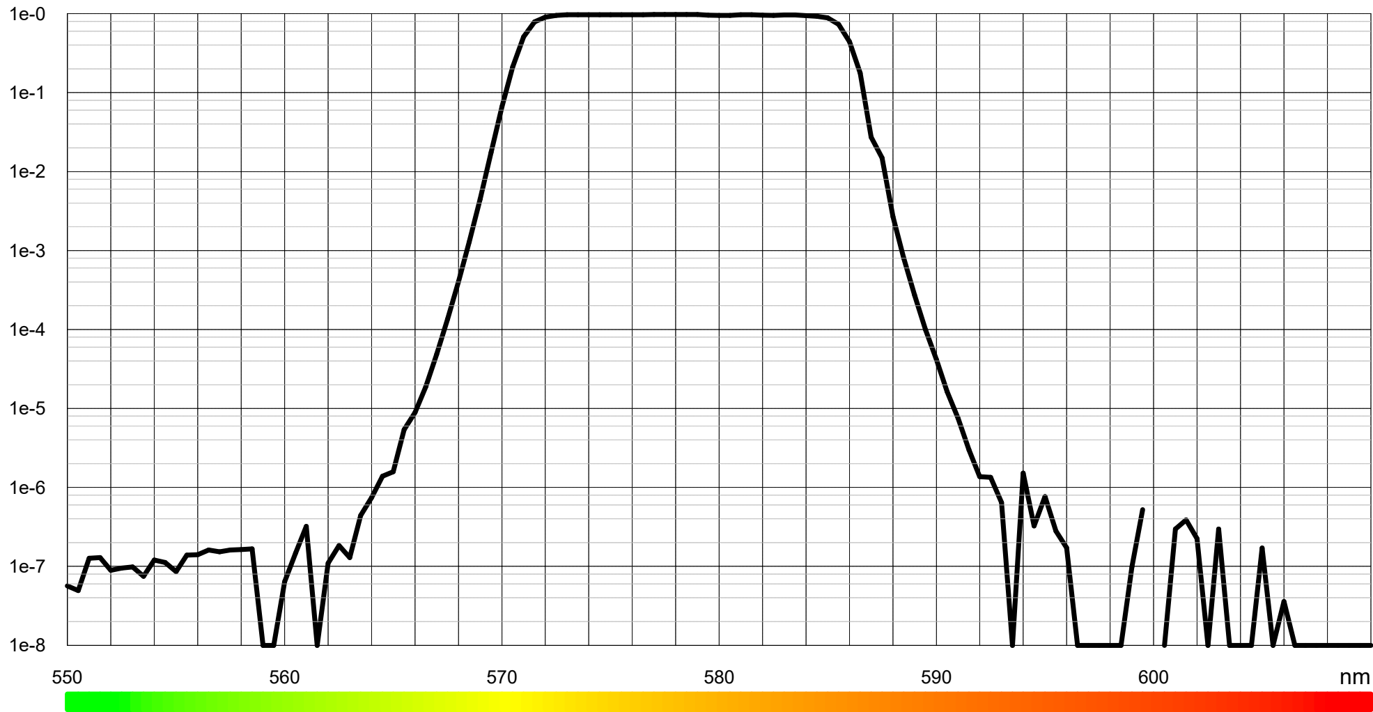
Typical transmission BP 579/16 (LF104542)
