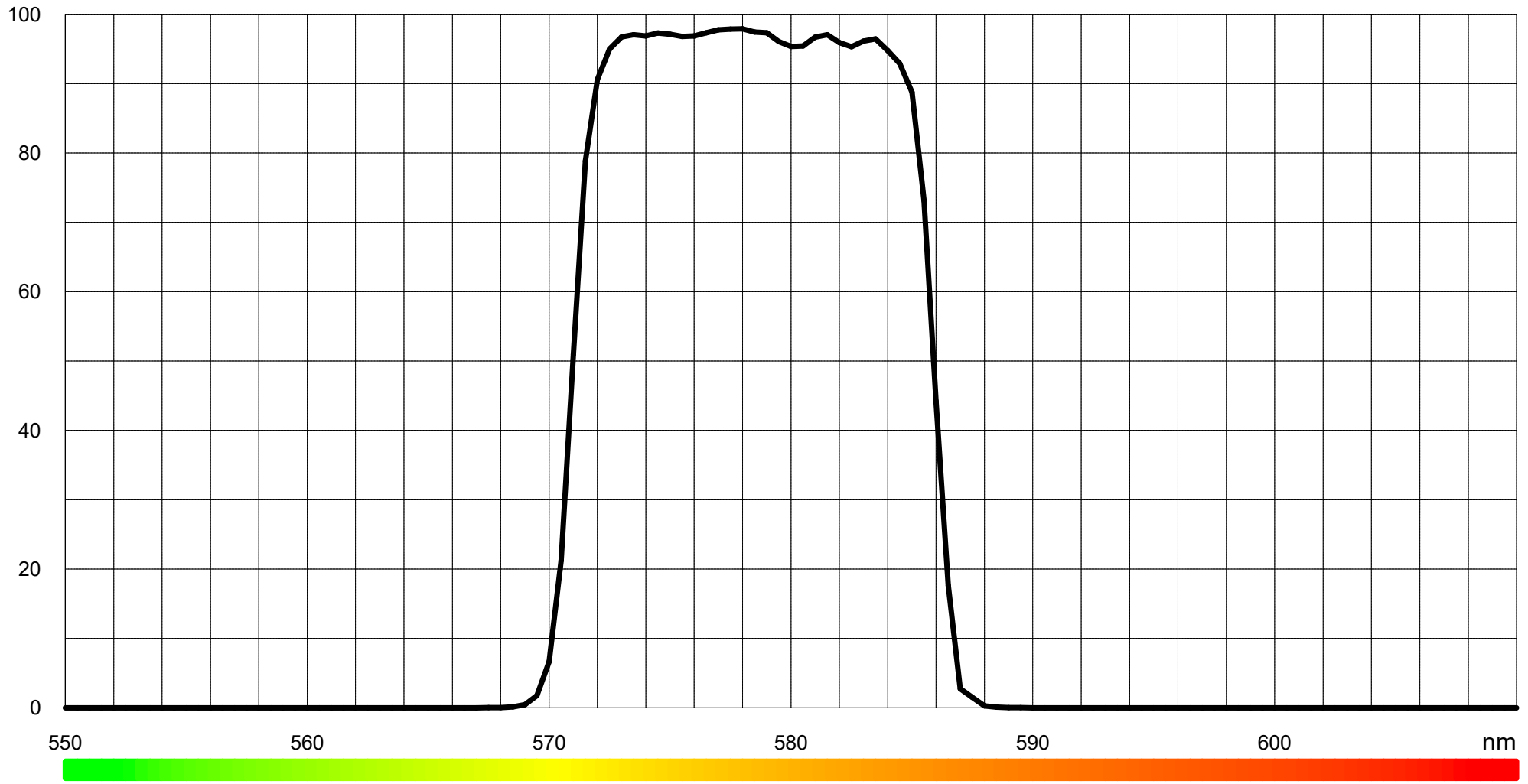
Typical transmission BP 579/16 (LF104542)
