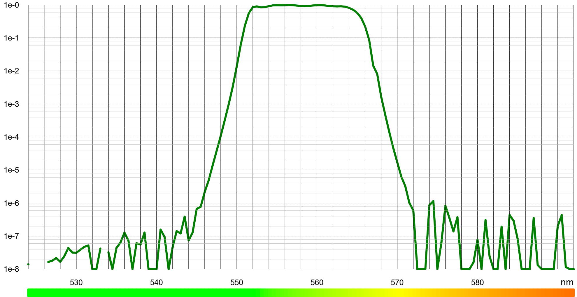
Typical transmission BP 558/14 (LF104548)
