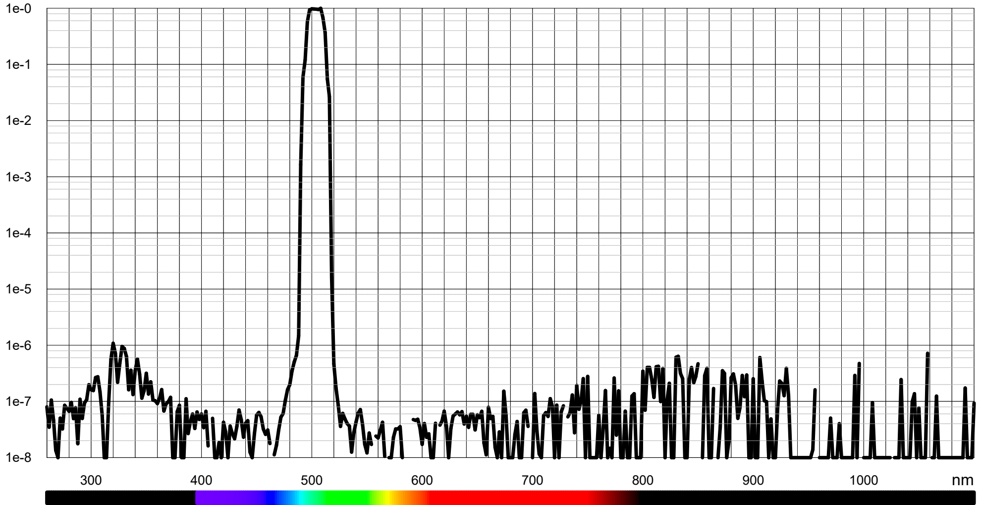
Typical transmission BP 505/16 (LF104540)
