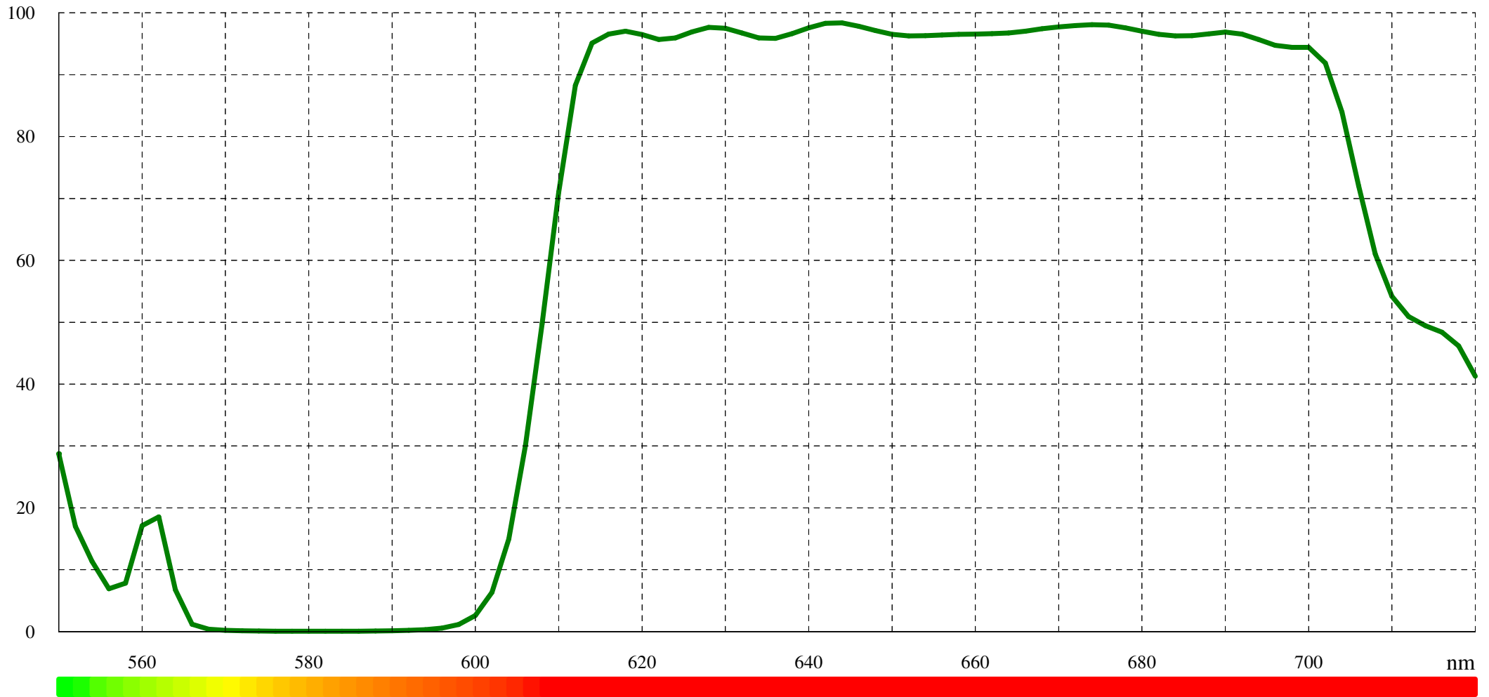
Typical transmission for TopPride™ DCLP 605 (LF101623)
