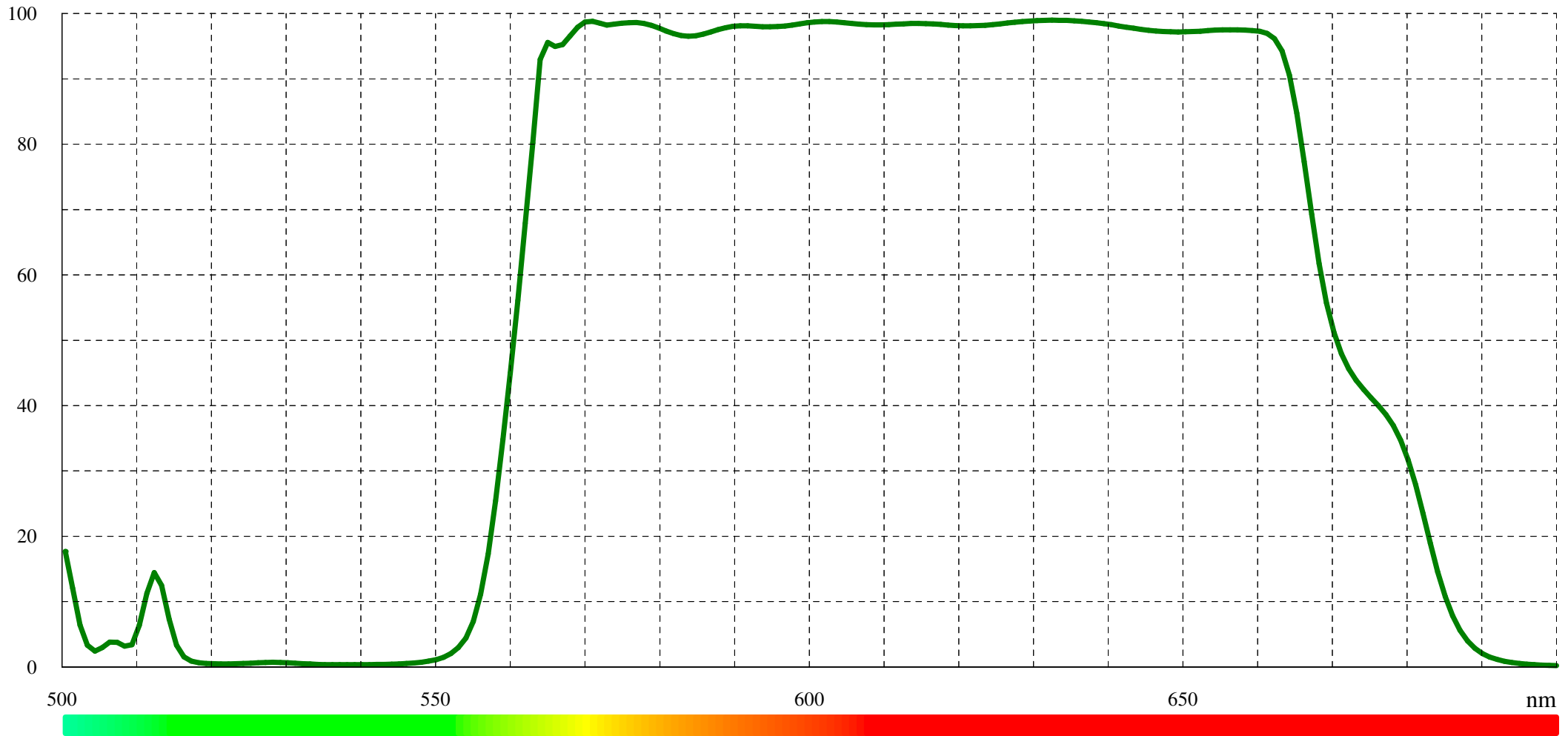
Typical transmission for TopPride™ DCLP 560 (LF101705)
