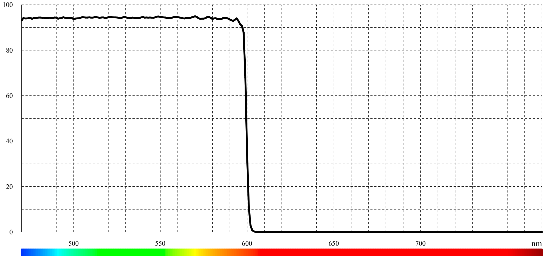
Typical transmission for SP 600 (LF101851)
