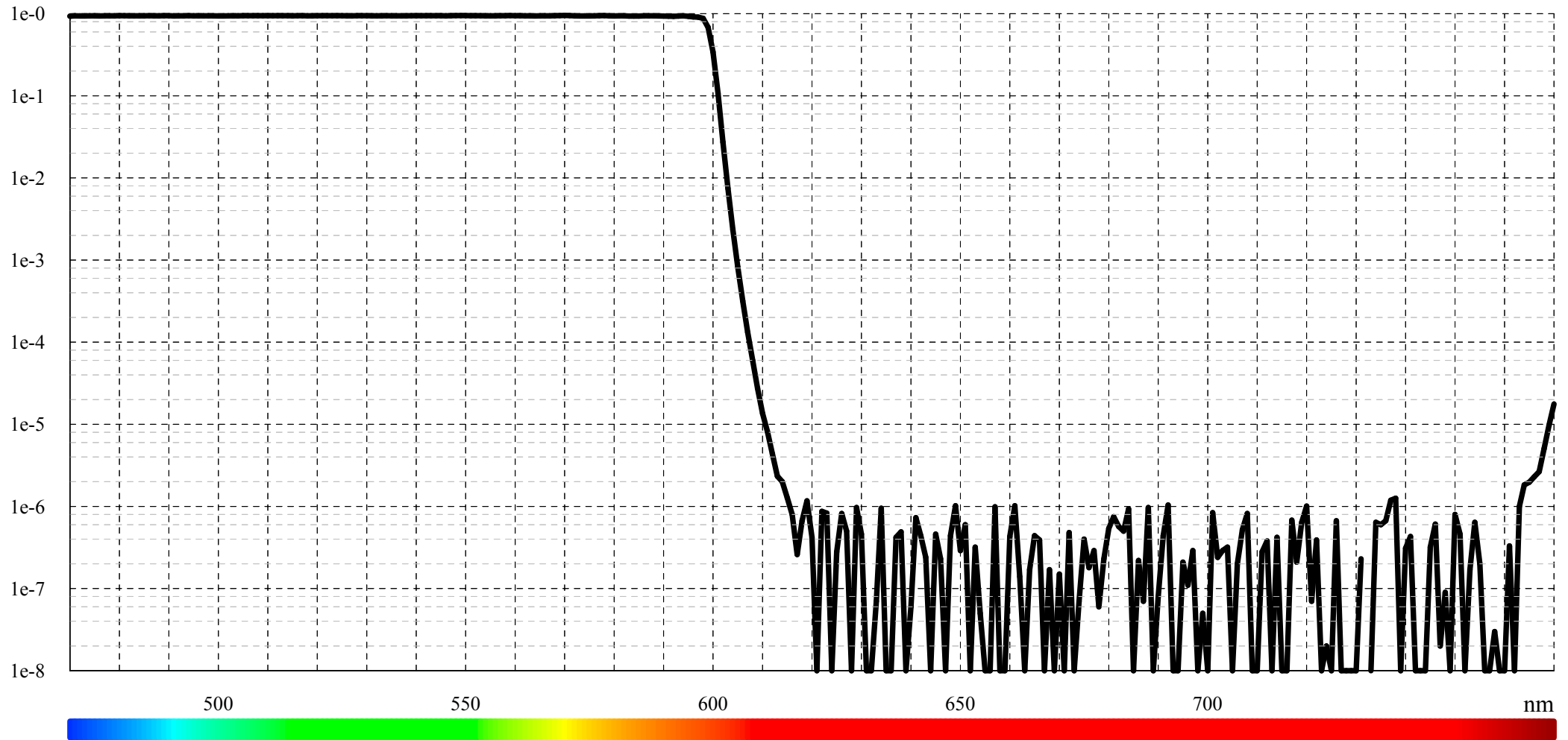
Typical blocking for SP 600 (LF101851)
