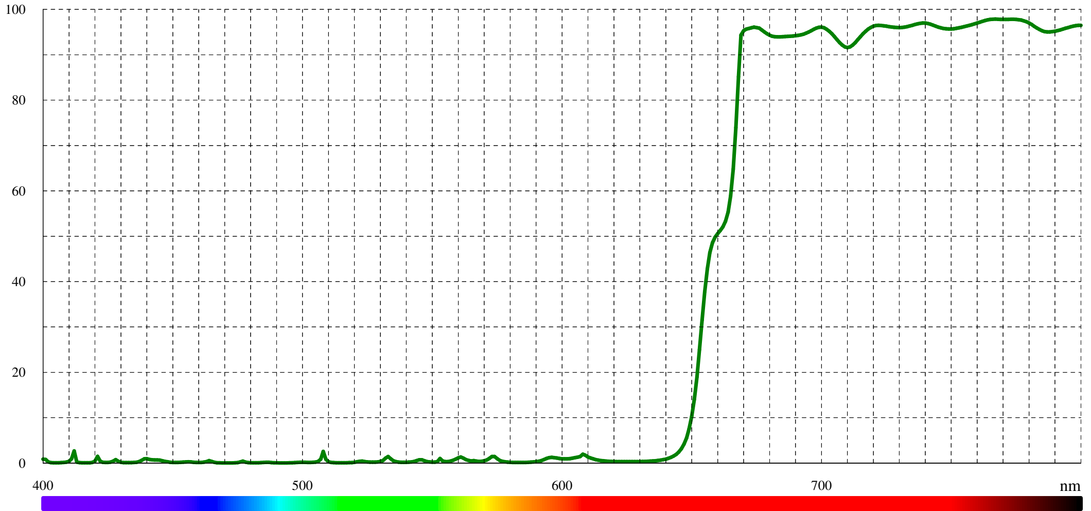
Typical transmission for DCLP 660 (LF101723)
