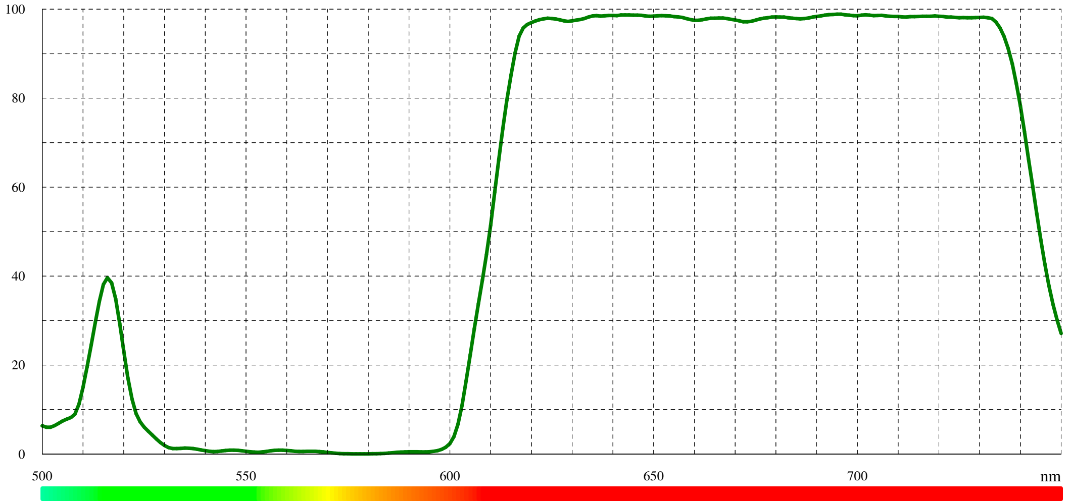
Typical transmission for DCLP 615 (LF101713)
