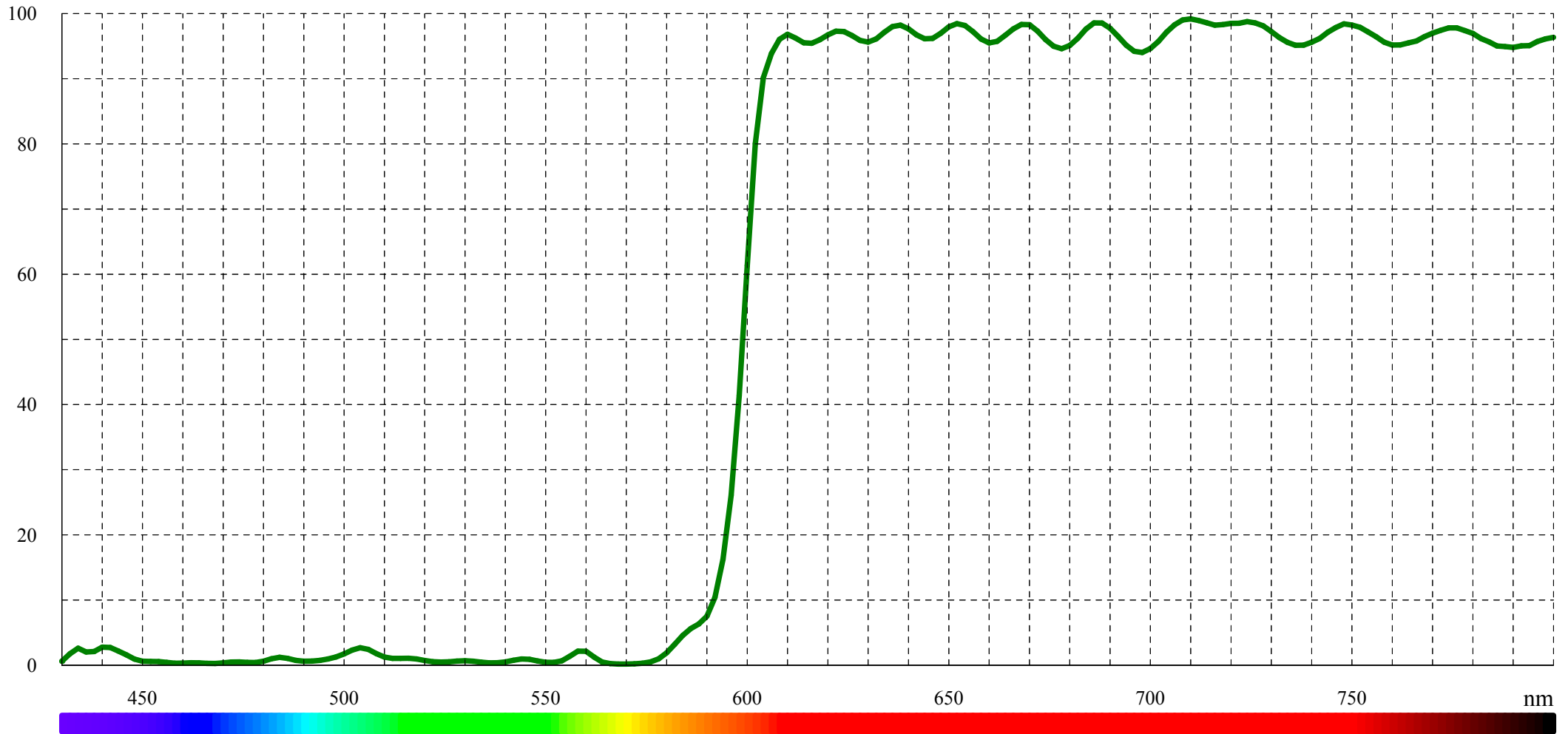
Typical transmission curve for DCLP 600 (LF101818)
