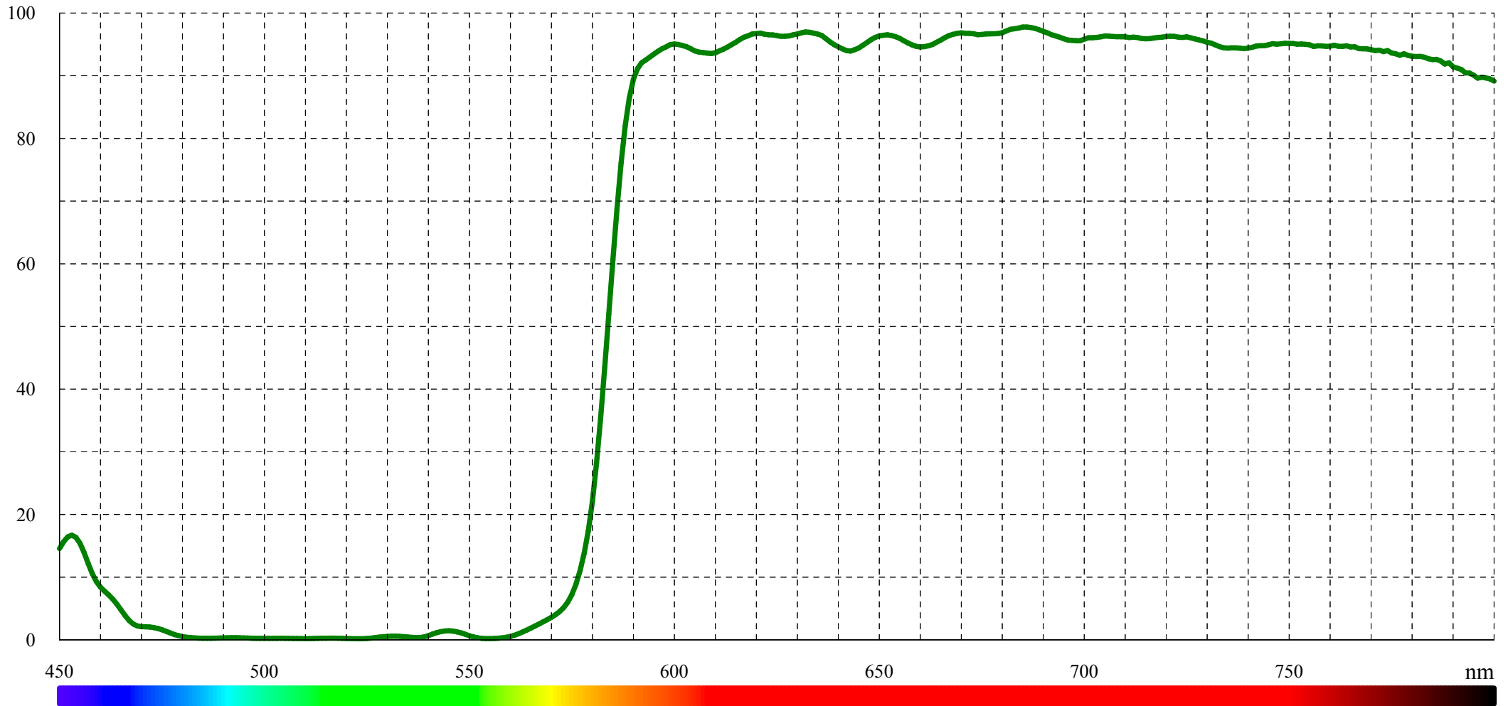
Typical transmission for DCLP 585 (LF101578)
