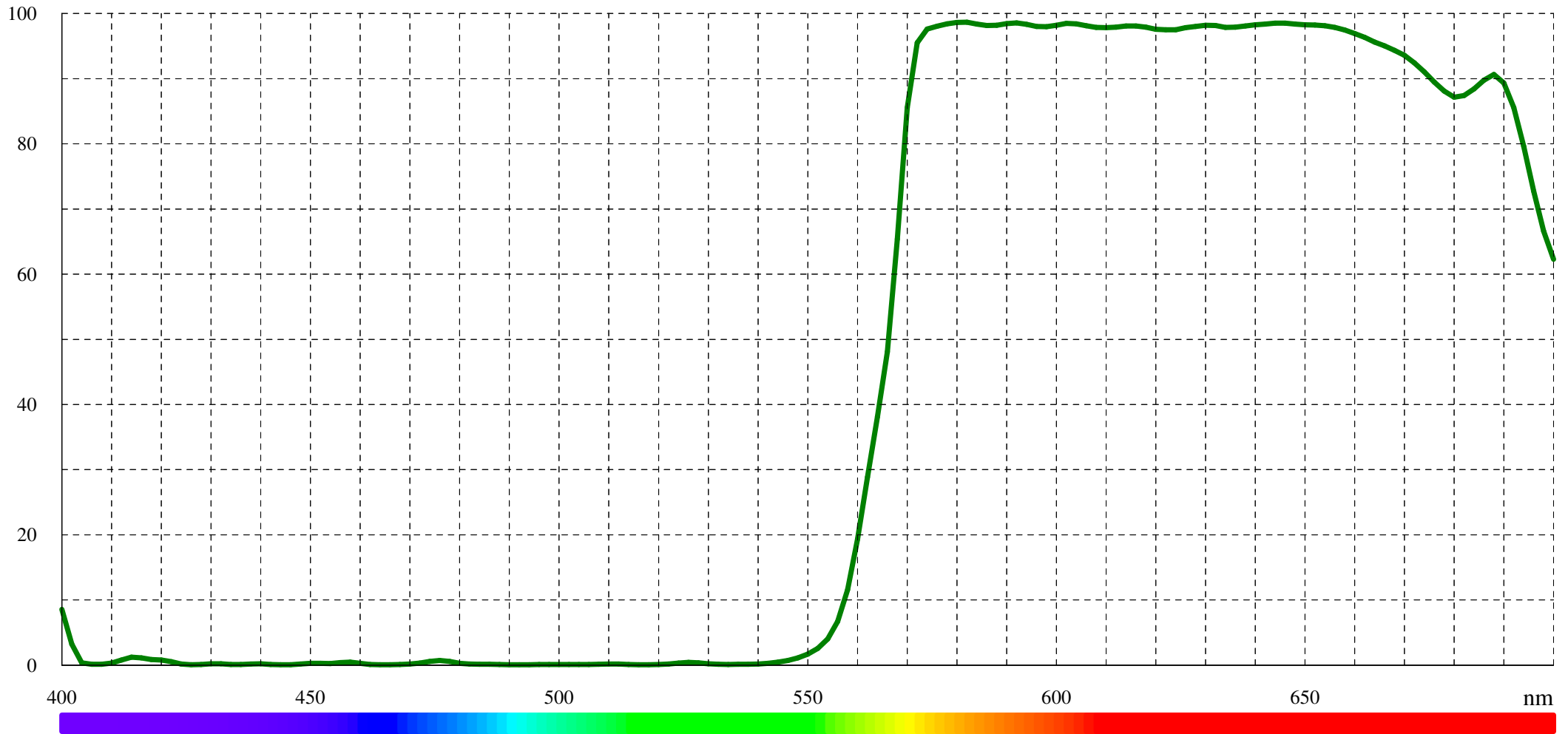
Typical transmission for DCLP 565 (LF101720)
