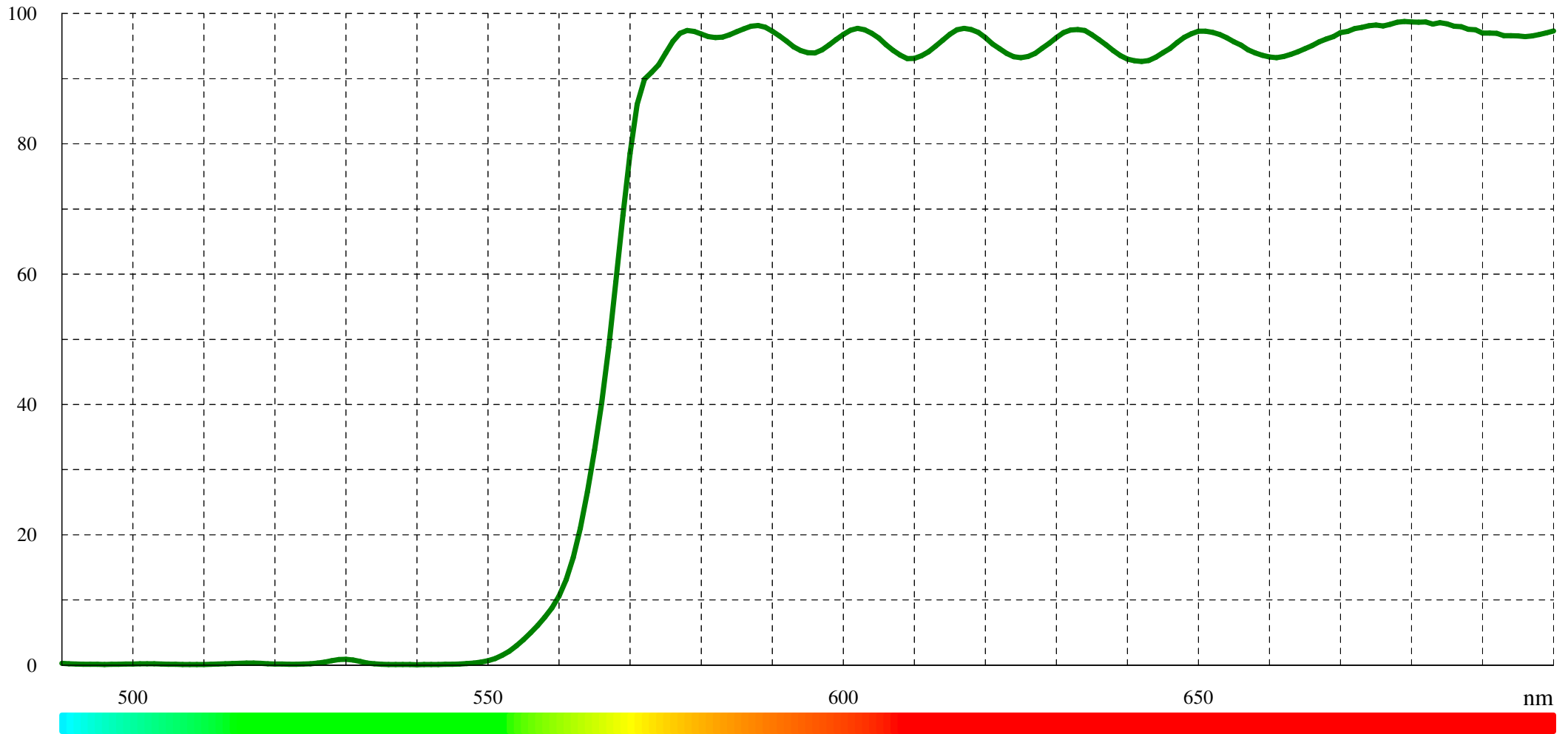
Typical transmission for DCLP 560 (LF101598)
