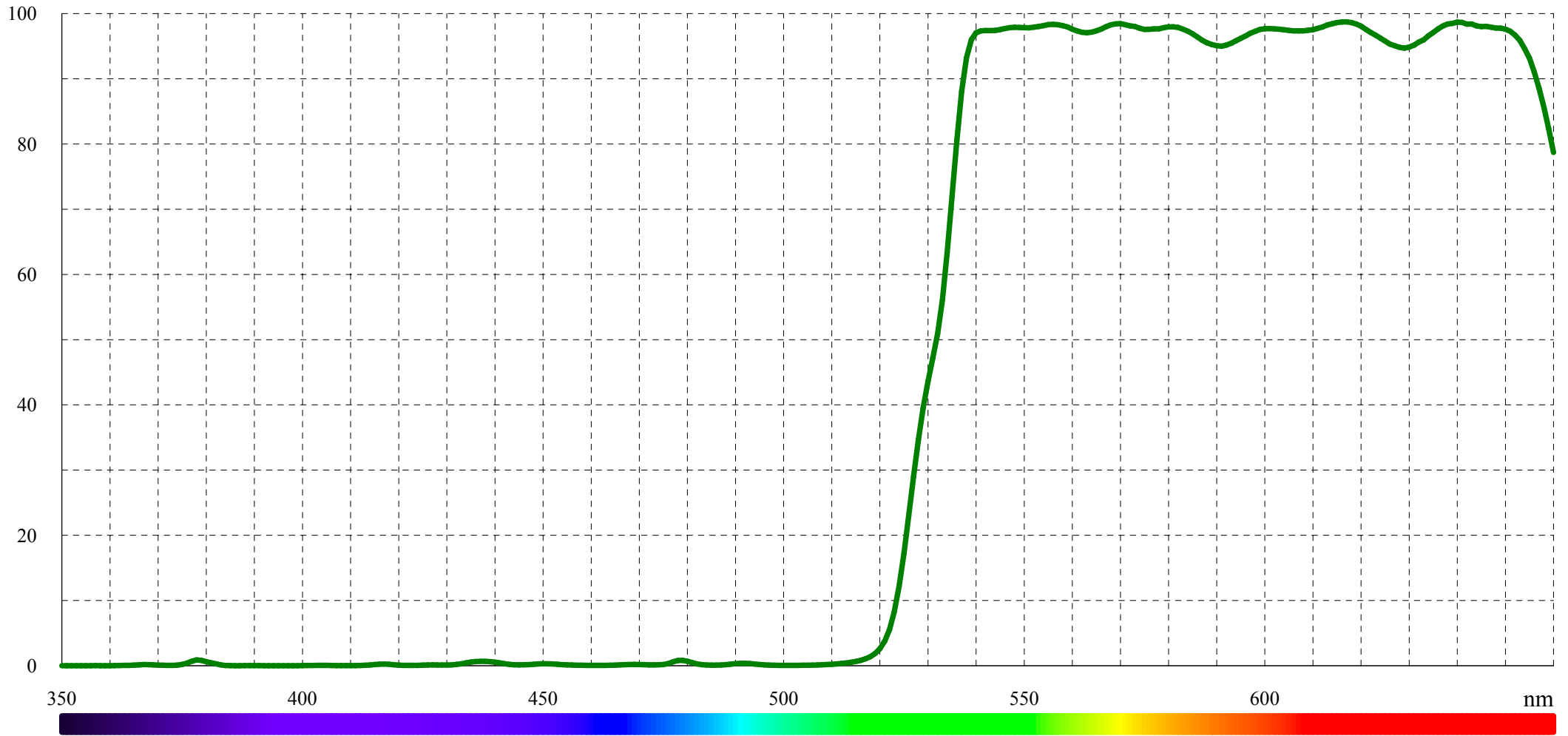
Typical transmission for DCLP 535 (LF102008)
