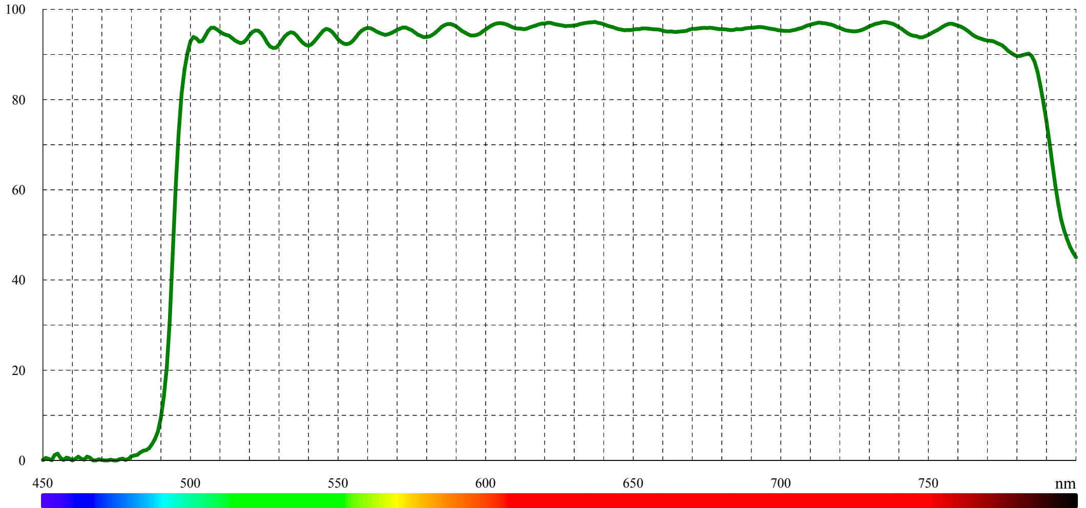
Typical transmission for DCLP 495 (LF102021)
