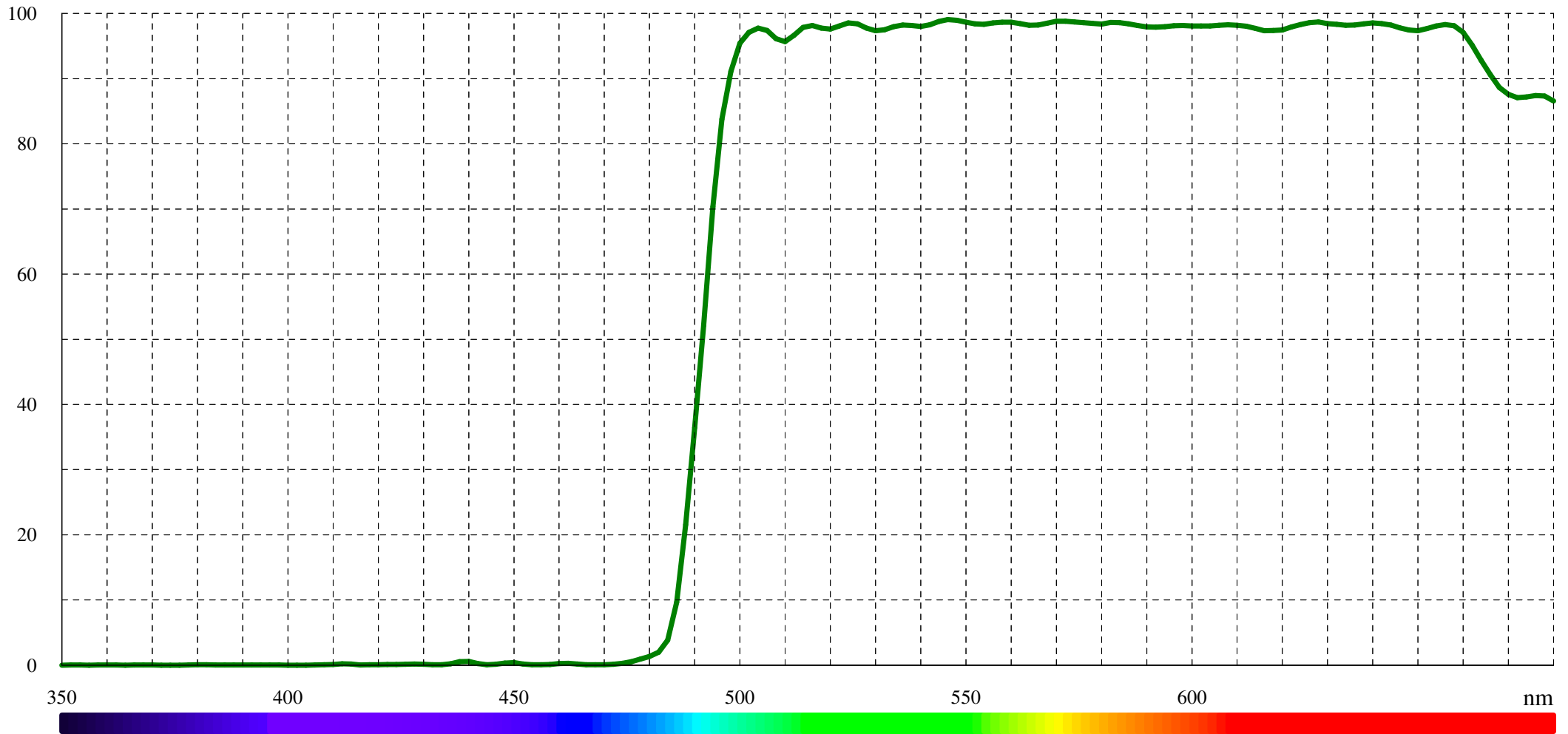
Typical transmission for DCLP 490 (LF101718)
