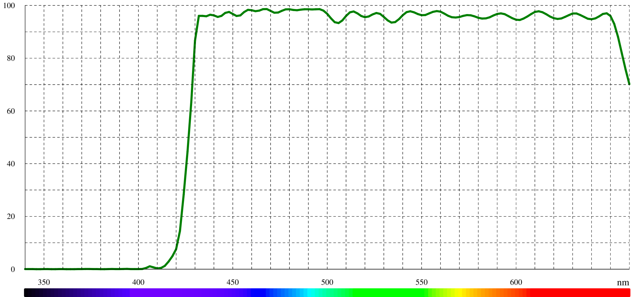
Typical transmission for DCLP 425 (LF101717)
