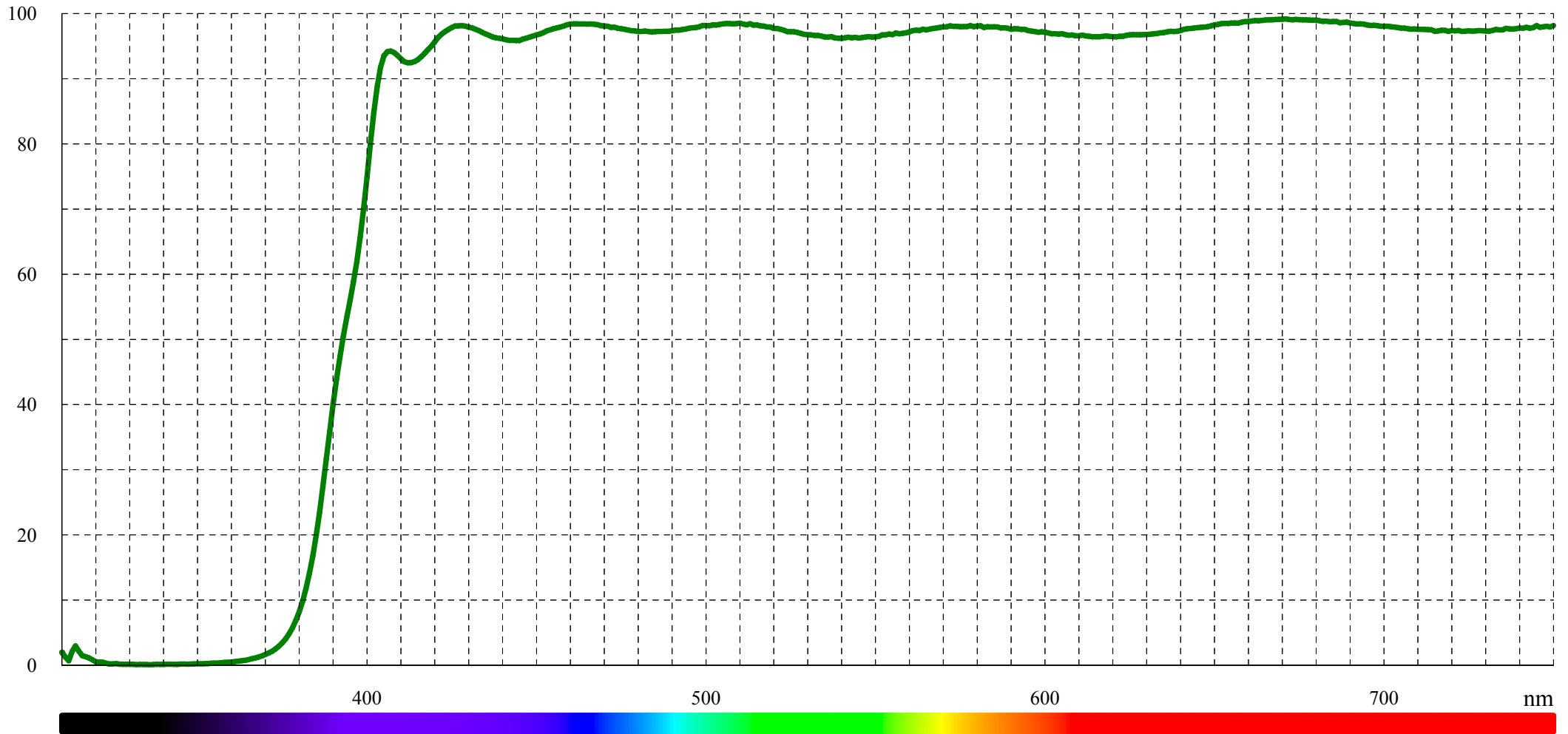
Typical transmission for DCLP 395 (LF101580)
